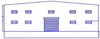
FRONT ELEVATION
