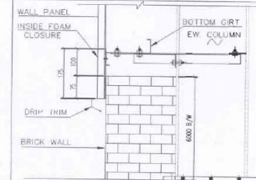
SECTION W-W (TYP) DRIP TRIM DETAILS (TYP)
