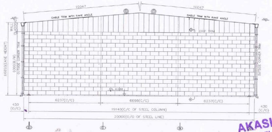
ENDWALL SHEETING ELEVATION : F.L. - 11 PANEL WALL METAL SHEET @ 50 THICK. COLOUR, COLOUR COATED PANEL CUSTOMER TO CONTAIN WALL SHEETING & FLASHING COLOUR.
