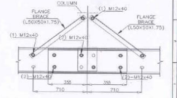
SECTION, X-X (TYP) GIRT LAP DETAIL (SHORT LAP)
