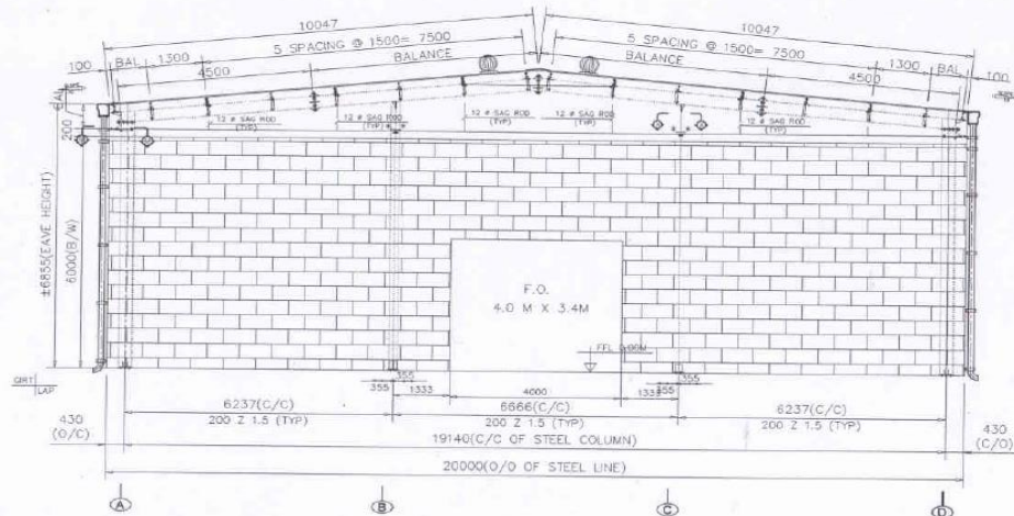
END FRAMING ELEVATION @ F.L. - 1 DOUBLE SIDED FLANGE BRACE
