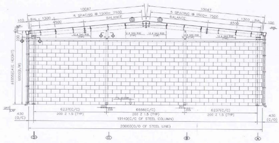
END FRAMING ELEVATION @ F.L. - 11 ♦♦ DOUBLE SIDED FLANGE BRACE
