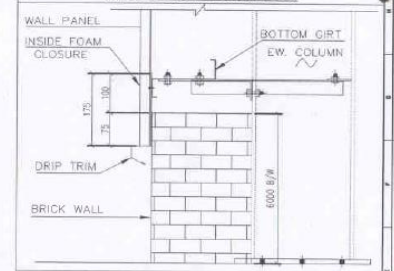
SECTION, W-W (TYP) DRIP TRIM DETAILS (TYP)
