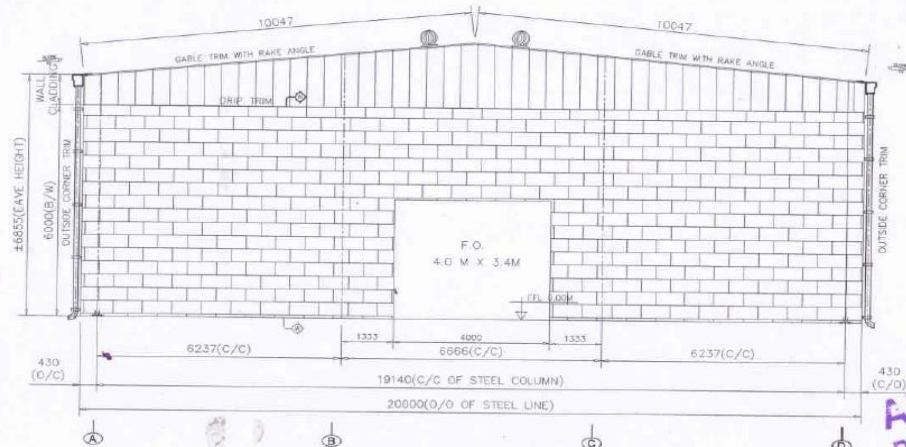
END WALL SHEETING ELEVATION: F.L. - 1 PANEL: WALL METAL SHEET 0.50 THK, COLOUR: COLOUR COATED PANEL CUSTOMER TO CONFIRM WALL SHEETING & EXTERIOR COLOUR
