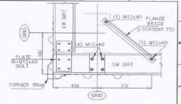
SECTION, M-M (TYP) (GIRT CONNECTION DETAILS @ CORNER)
