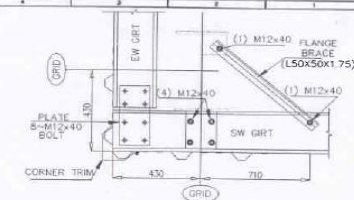
SECTION M-M (TYP) GIRT CONNECTION DETAILS @ CORNER
